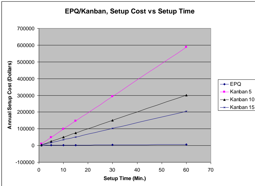
Figure 3: EPQ/Kanban, Annual Setup Cost vs Setup Time
