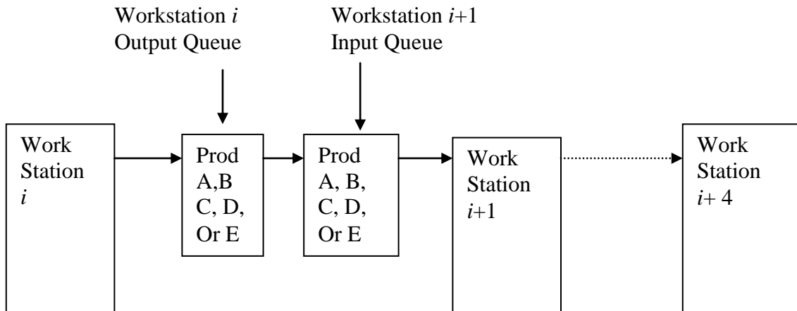
Figure 2: EPQ Simulation Model
